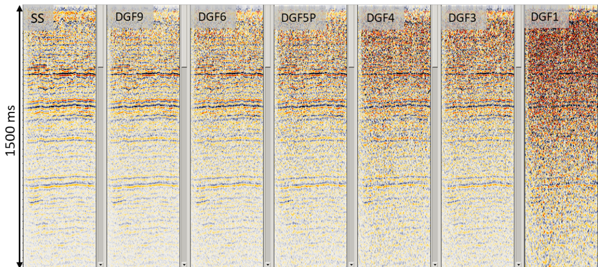
Figure 3. True amplitude migrated stacks of a selection of DGF designs. Vertical axis is two-way time.
