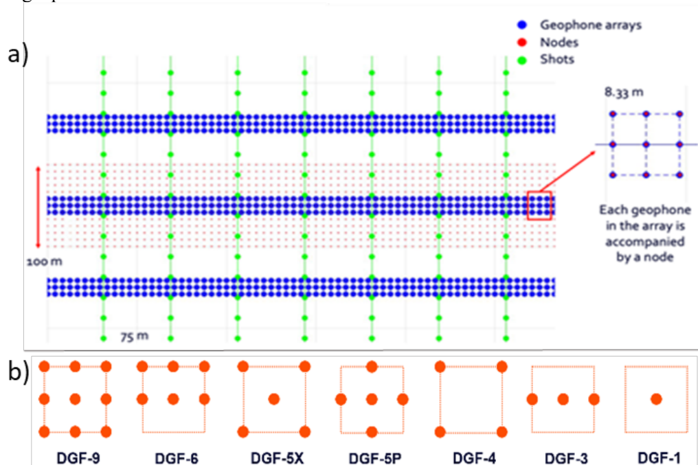
Figure 1. Schematic representation of the acquisition geometry including shot points (green dots), geophone arrays (blue dots) and nodes (red dots) (a) and DGF patterns tested in the field trial (b).
