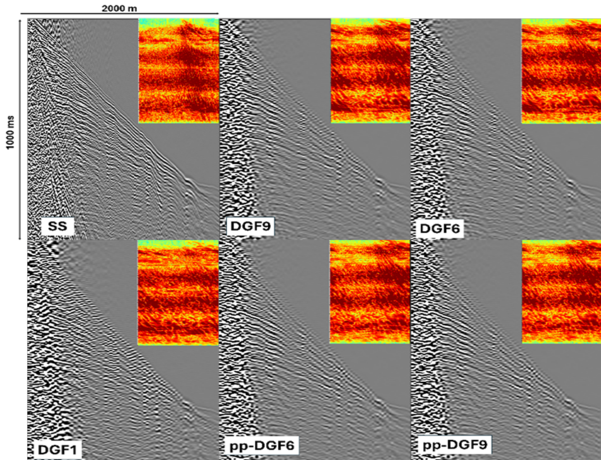
Figure 2. Raw shot gathers and associated FK spectra of the single sensor (SS) data and some of the DGF and pp-DGF designs tested in this study.
